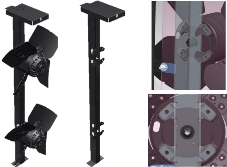
Figure 4: Fan bracket details
