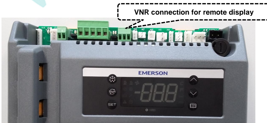
Figure 12: VNR connection for the remote display
