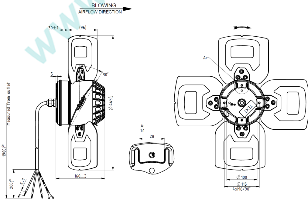
Figure 3: Fan details and dimensions
