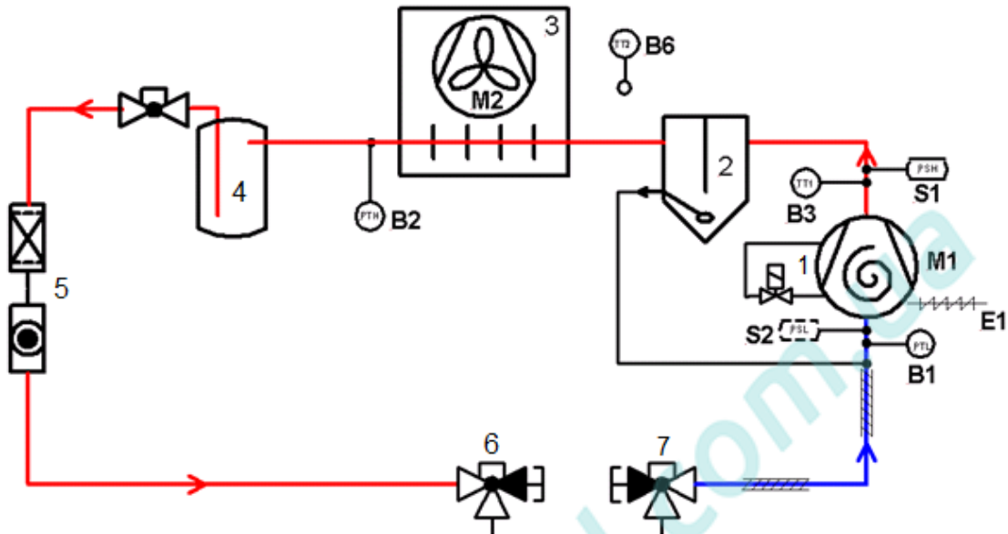
Figure 6: P&I diagram for ZXDI units
